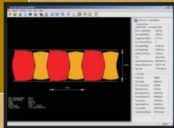
Blanknest will optimize layouts with up to two different blanks
