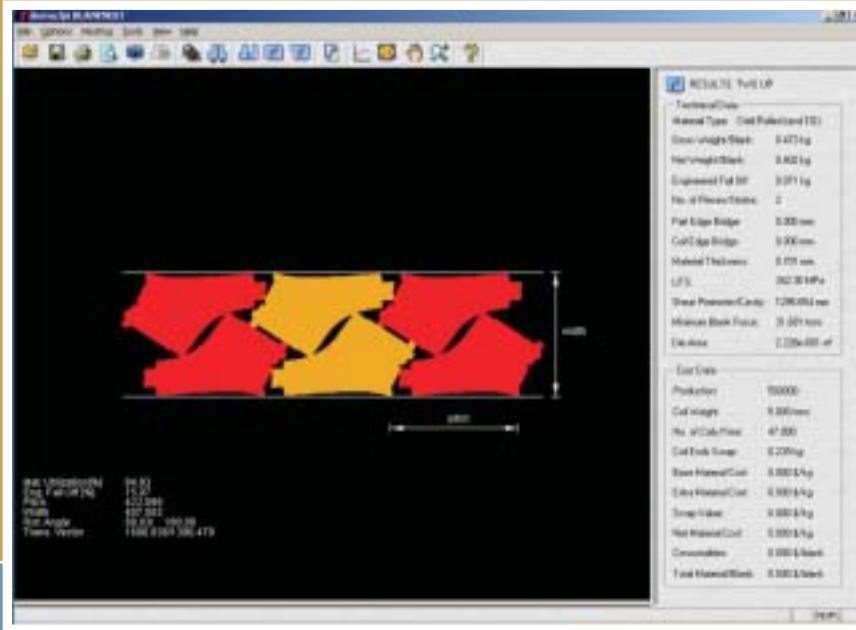
Optimal Blank Nesting Layout
