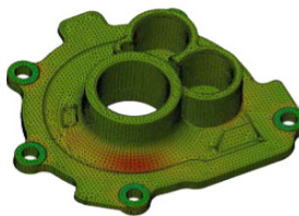
FIGURE 13: VYNCOLIT, BASED IN GENT, BELGIUM, USES SOLIDWORKS TO CHECK THE PERFORMANCE OF COMPONENTS MADE OUT OF PHENOLICS MATERIAL. PHENOLICS MATERIALS HAVE A NUMBER OF PHYSICAL PROPERTIES THAT MAKE THEM IDEAL FOR MANY APPLICATIONS, WHICH HAVE TRADITIONALLY BEEN SERVED BY METAL OR THERMOPLASTICS, IN INDUSTRIES SUCH AS ELECTRONICS AND AUTOMOTIVE.
